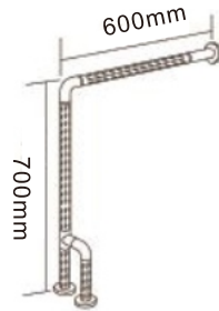
UP-D6070B 材质：尼龙和金属管件 配置：普通连接件 颜色：白色和黄色 Material: nylon and metal fittings Configuration: general connector Color: white and yellow
