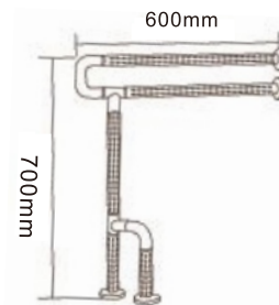
UP-D6070D 材质：尼龙和金属管件 配置：普通连接件 颜色：白色和黄色 Material: nylon and metal fittings Configuration: general connector Color: white and yellow
