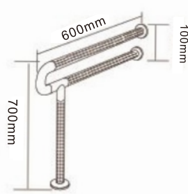
UP-D6070C 材质：尼龙和金属管件 配置：普通连接件 颜色：白色和黄色 Material: nylon and metal fittings Configuration: general connector Color: white and yellow
